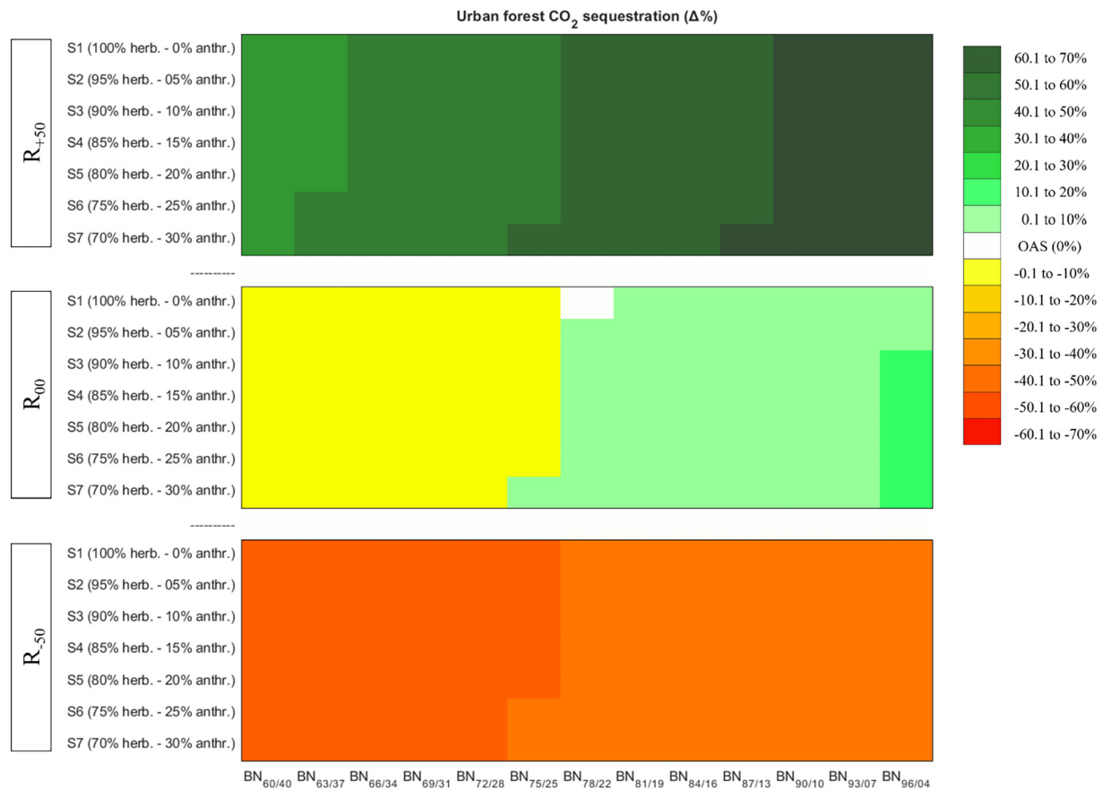
Fig. 4. Map of \Delta\text{CO}_2 sequestration between OAS and 272 AAS. The comparison was proposed considering only the reference, the maximum (+50%) and the minimum (-50%) surface to be forested included in the analysis and evaluating \Delta\text{CO}_2 sequestration grouping scenarios by 10% classes.
