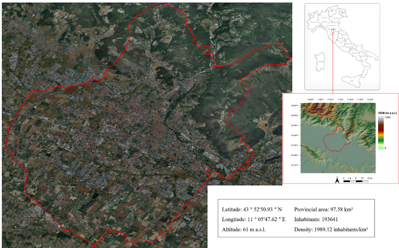
Fig. 1. Localization in Italy, orographic (DEM-Digital Elevation Model) and geographical information of Municipality of Prato.
