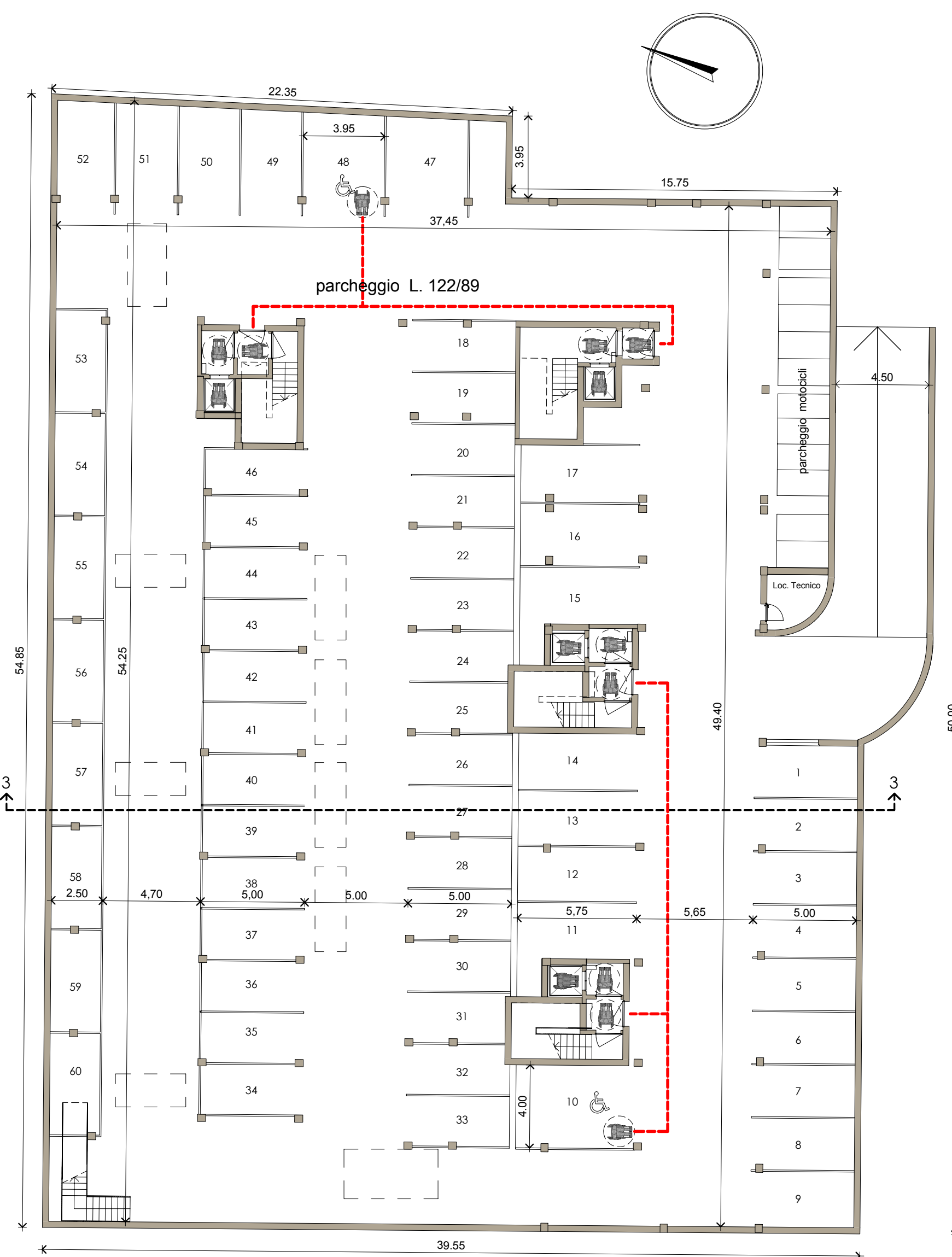
PIANO INTERRATO
